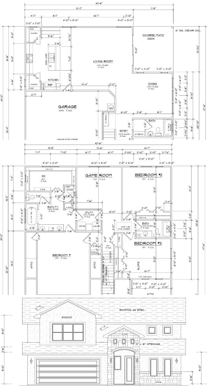
FRONT ELEVATION
